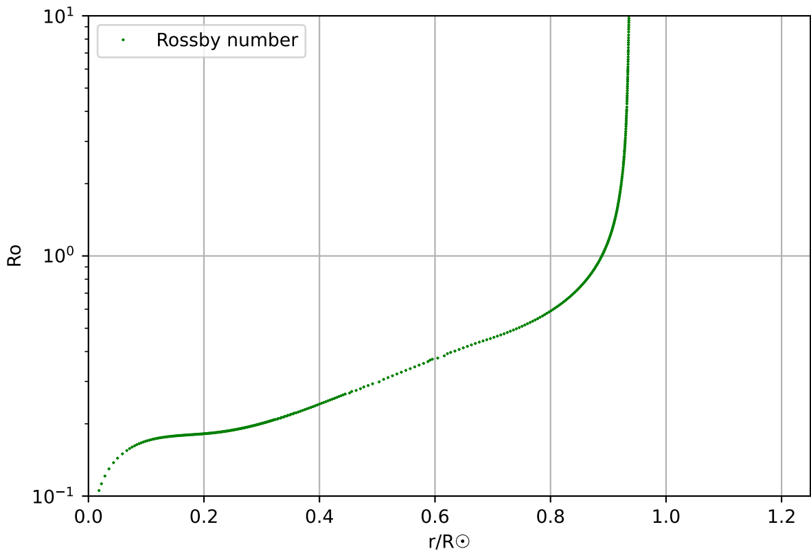
Rossby number, profile 138, age 2.43 \times 10^9
